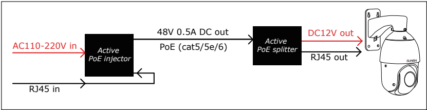
Active PoE Injector/Splitter are allowed if you use PoE to power non-PoE camera.
