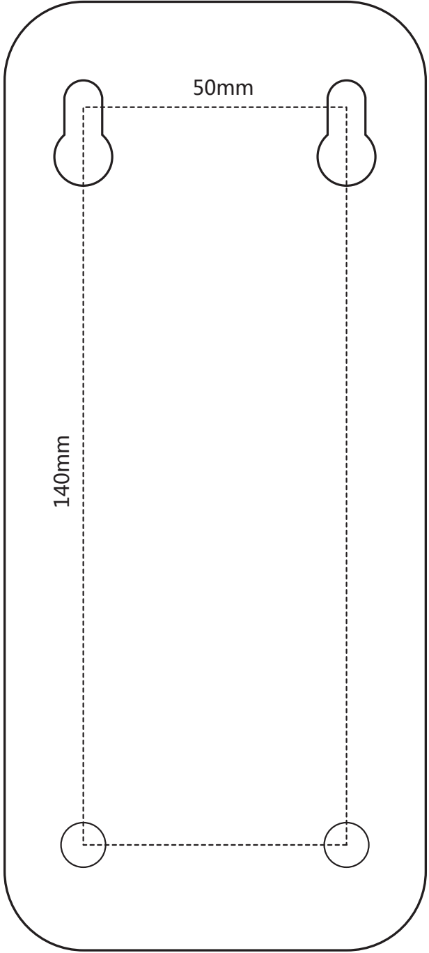
SUNBA 601 PTZ Bracket
